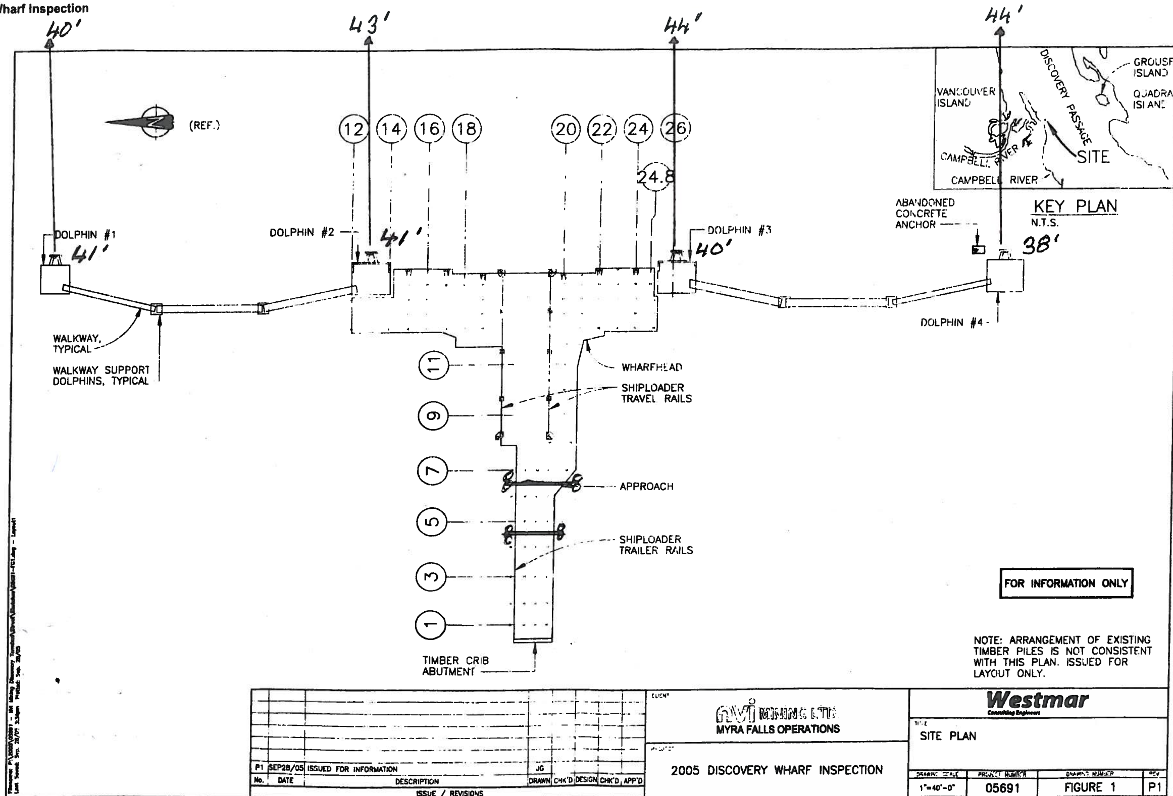
FIGURE 2-1: Site Plan
